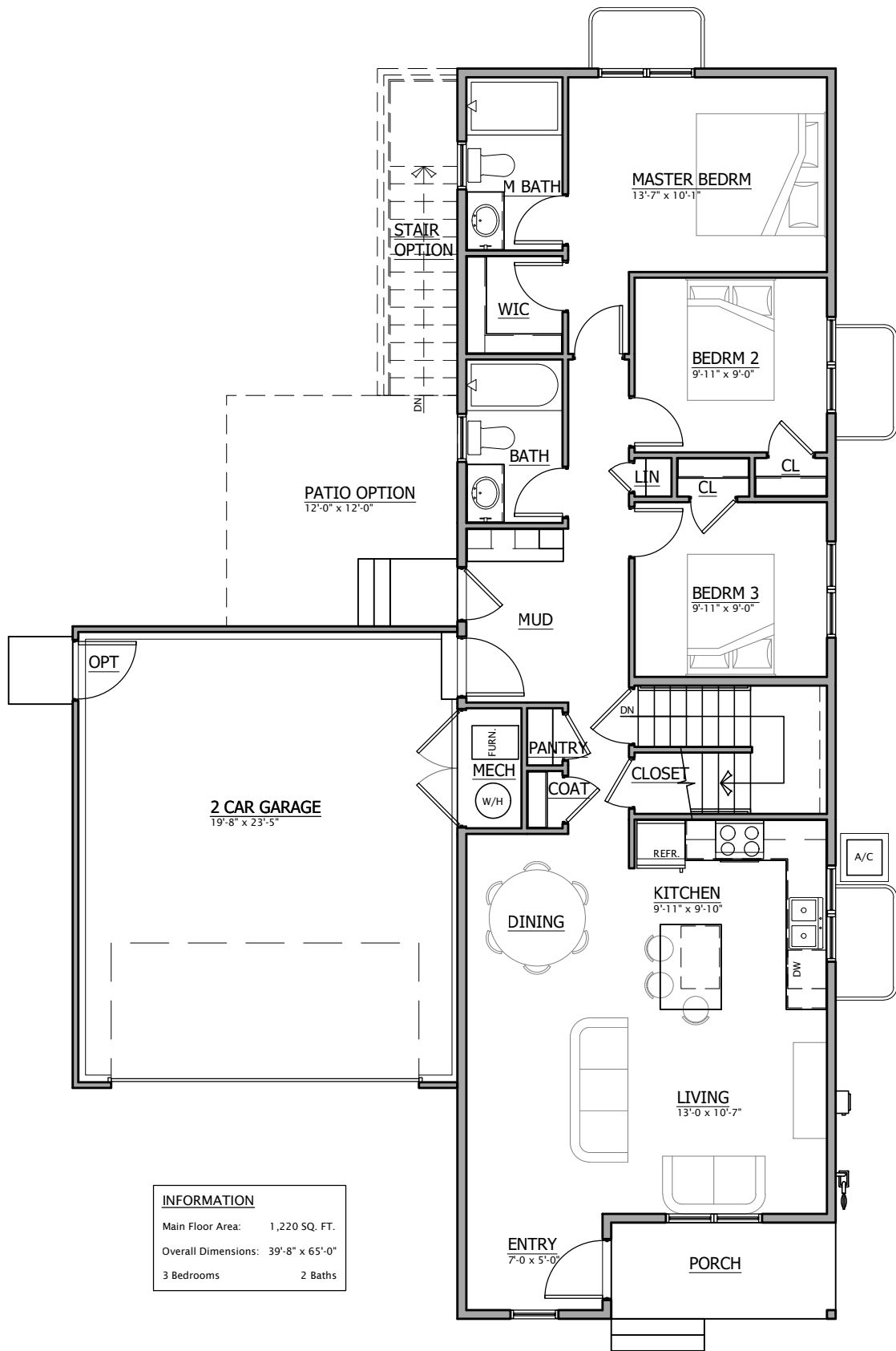
EAGLE LANDING 1220 - 3 BEDROOM STANDARD MAIN FLOOR PLAN © IRONTOWN HOMES
