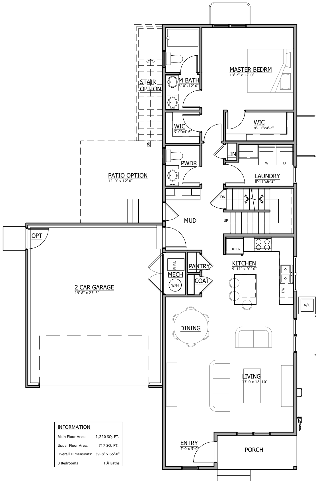
EAGLE LANDING 1976 - 3 BEDROOM OPTIONAL MAIN FLOOR PLAN © IRONTOWN HOMES
