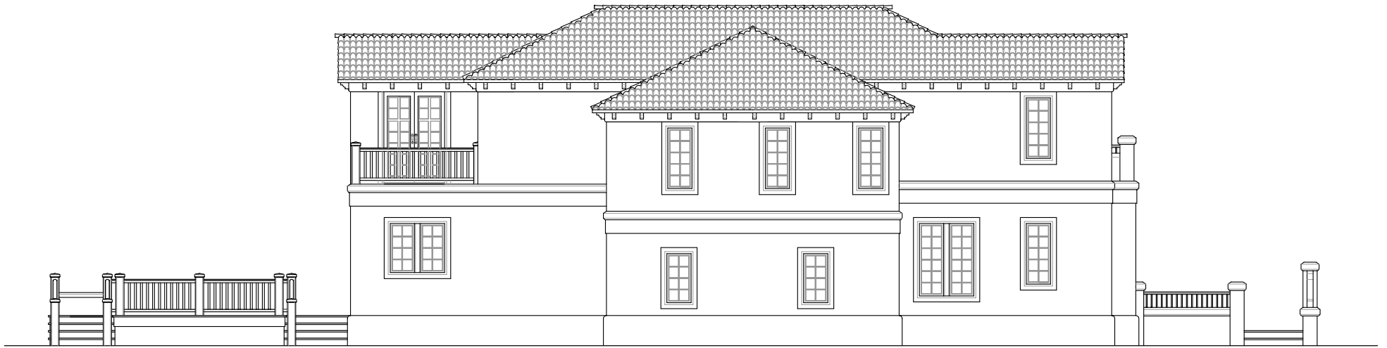
FIORENZA (c), LEFT ELEVATION, FACING
